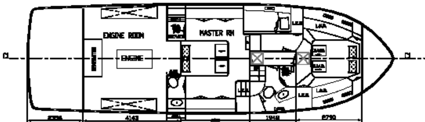
Integrity Grand Sedan 530GS 16.10x4.70x1.50 Meter Engine 1x Scania 700 HP
